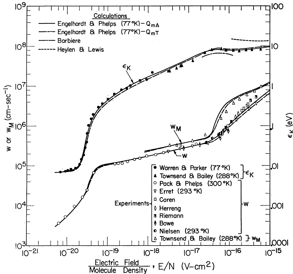
FIG. 2. Drift velocity w , magnetic drift velocity w_M , and characteristic energy \epsilon_K for electrons in argon as a function of E/N . Below \epsilon_K=0.5 eV the experimental data shown are for gas temperatures T_g of 77° and 87°K as discussed in the text. Above \epsilon_K=0.5 eV and for T_g \leq 300^\circ\text{K} the values of w , w_M , and \epsilon_K are insensitive to T_g . The solid and dashed curves represent our calculated results using Q_{mA} and Q_{mT} , respectively; the points represent the various experimental results.
