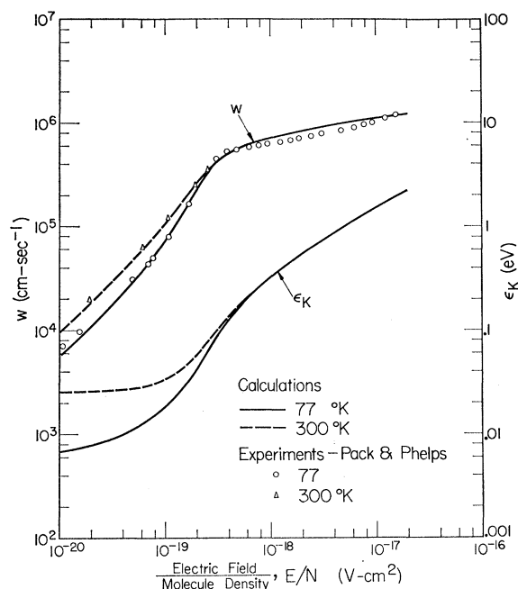
FIG. 5. Drift velocity w and characteristic energy \epsilon_K for electrons in a mixture of 1.5% H_2 in Ar as a function E/N . The solid lines represent our calculations for T_g = 77^\circ K and the dashed ones for T_g = 300^\circ K . The experimental results of Pack (Ref. 5) are shown as points.
