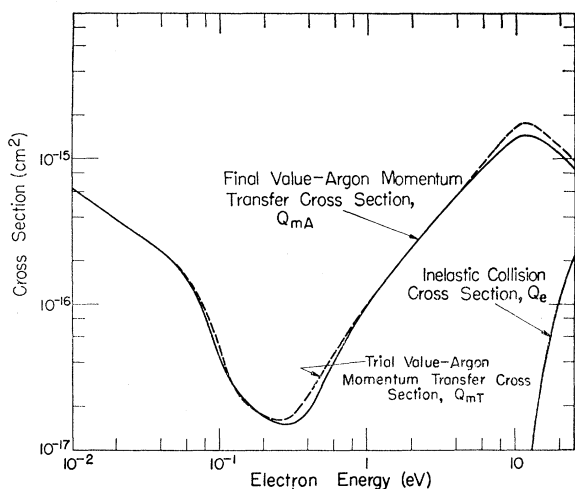
FIG. 1. Momentum transfer and inelastic collision cross sections for electrons in argon as a function of electron energy in eV. Q_{mA} (solid line) is our final value of the momentum transfer cross section and Q_{mT} (dashed line) is a trial value.
