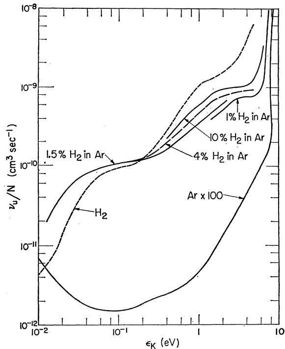
FIG. 6. Calculated energy exchange frequency \nu_u/N for Ar, H 2 , and 1, 1.5, 4, and 10% H 2 in Ar at T_g = 77^\circ\text{K} as a function of \epsilon_K in eV. In the case of the mixtures \nu_u/N is obtained using Eq. (3). For Ar, \nu_u/N is shown increased by a factor of 100.
