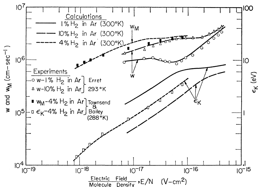
FIG. 4. Drift velocity w , magnetic drift velocity w_M , and characteristic energy \epsilon_K as a function of E/N for electrons in mixtures of 1, 4, and 10% H_2 in Ar. The solid, dashed, and dotted curves represent our calculated results for 1, 4, and 10% H_2 in Ar, respectively. The various experimental data are shown as points.
